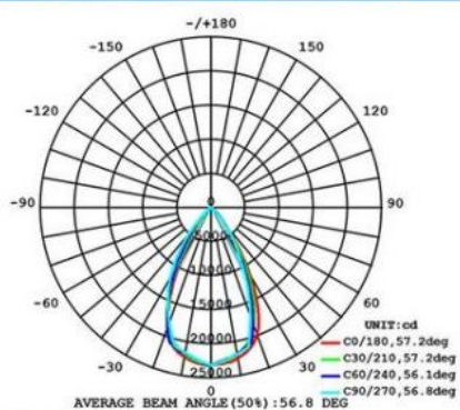
HB-H150W 6000K Light distribution curve
