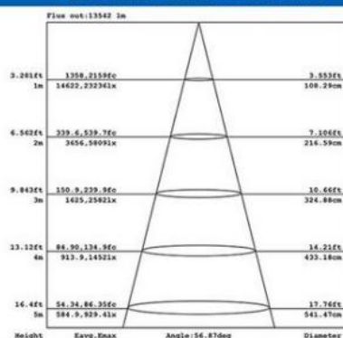
HB-H150W 6000K Illumination curve
