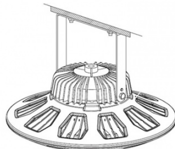
3. Mount Surface Hanging
